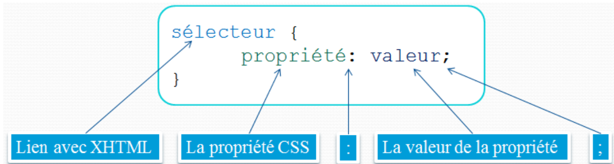
Figure 2 – Syntaxe CSS
